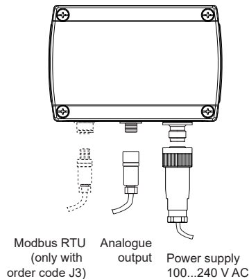
Fig. 34 Polycarbonate enclosure
