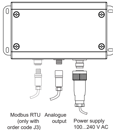
Fig. 35 Stainless steel enclosure
