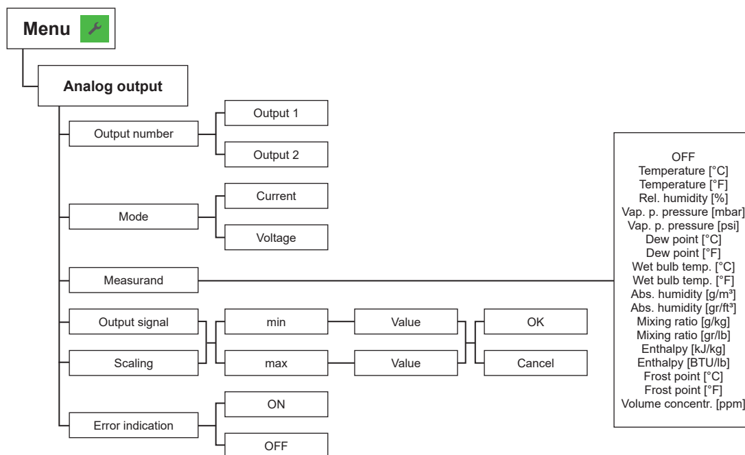
Fig. 50 Analogue output
