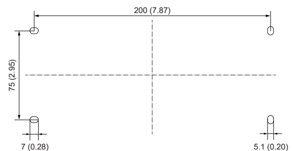
Fig. 26 Drilling pattern of stainless steel enclosure
